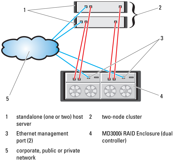
Figure 6. Cabling iSCSI Direct-Attached Clusters
